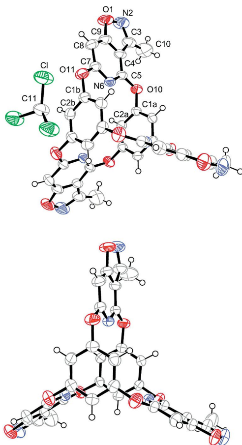
Figure 2. Two views of the ORTEP drawing of compound 6 ·CHCl 3 (50% probability thermal ellipsoids). The site-occupation factor for the reported chloroform molecule is 0.55(4). In the bottom view, the chloroform molecule is omitted for clarity.
