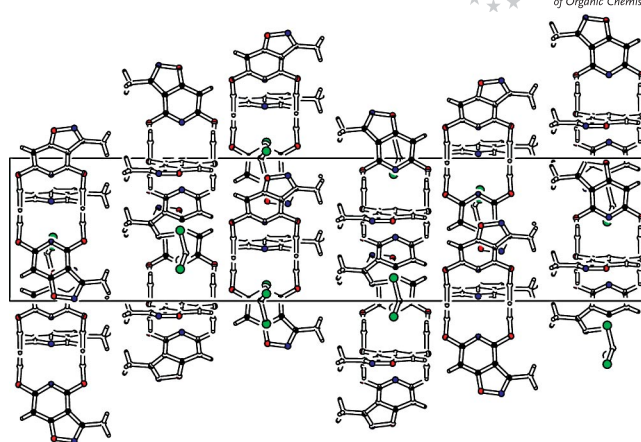
Figure 3. Crystal packing views along the x axis of 6 ·CHCl 3 .
