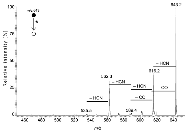
Figure 1. APCI MS–MS spectrum of [5 + H]^+ ( m/z = 643 ) selected as the precursor ion.
