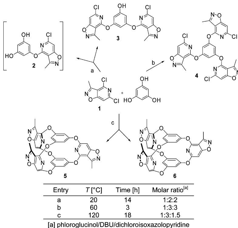
Scheme 1. Experimental conditions for the synthesis of compounds 3–6.
