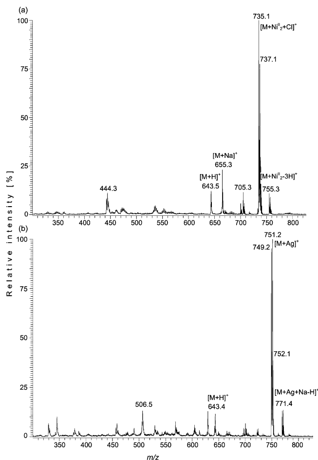
Figure 6. Electrospray spectra (positive mode) obtained by mixing 5 with NiCl 2 (a) or AgNO 3 (b).
