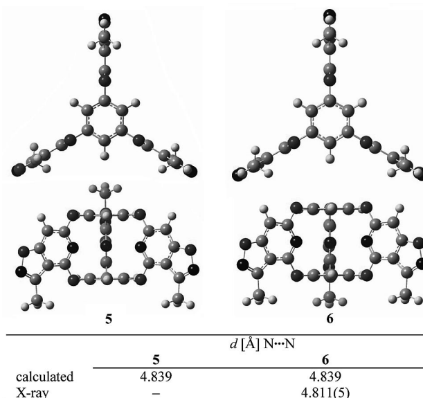
Figure 4. Two different views of the energy-minimized structures [B3LYP/6-31G(d,p)] of compounds 5 and 6 .
