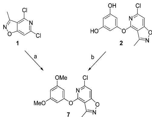
Scheme 2. Synthesis of dimethoxy derivative 7 . Reagents and conditions: (a) 3,5-dimethoxyphenol, DBU, DMSO, r.t.; (b) excess diazomethane, methanol.
