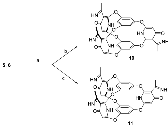
Scheme 3. Catalytic hydrogenation of bicyclooxacalix[4]arenes. Reagents and conditions: (a) \text{H}_2 , 10% Pd on carbon, ethyl acetate, 60 psi, r.t.; (b) from 5 ; (c) from 6 .
