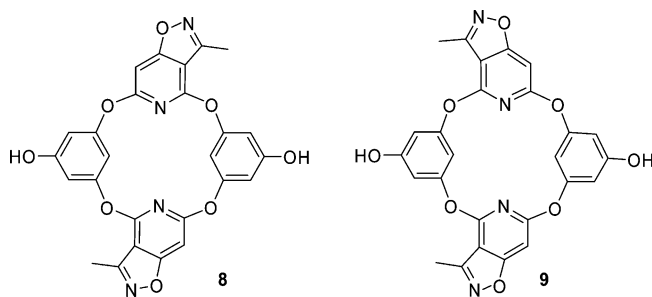
Figure 5. Structures of calixarenes 8 and 9 .
